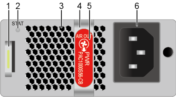
Figure 5-53 Panel of the PAC1000S56-CB
