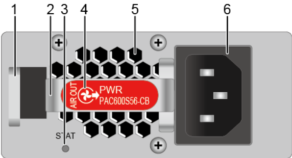
Figure 5-49 Panel of the PAC600S56-CB
