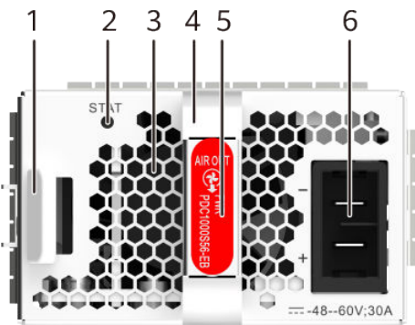
Figure 5-65 Panel of the PDC1000S56-EB
