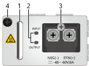
Figure 5-35 Panel of the ES5M0PSD1700
