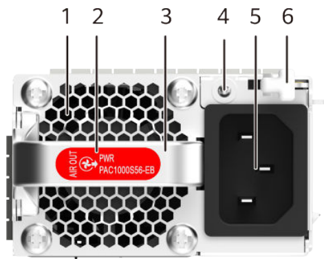
Figure 5-59 Panel of the PAC1000S56-EB
