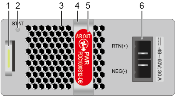
Figure 5-63 Panel of the PDC1000S12-DB
