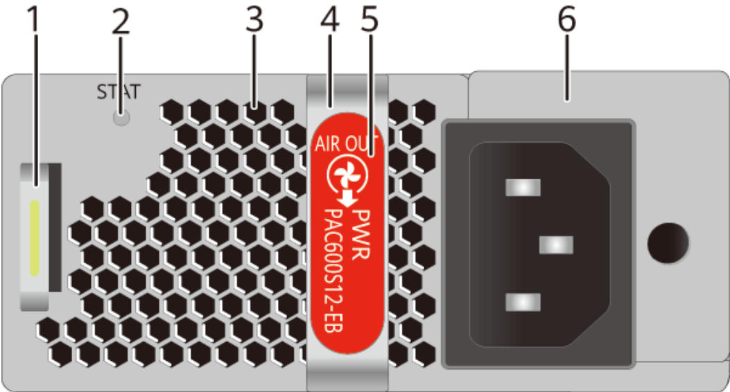
Figure 5-47 Panel of the PAC600S12-EB
