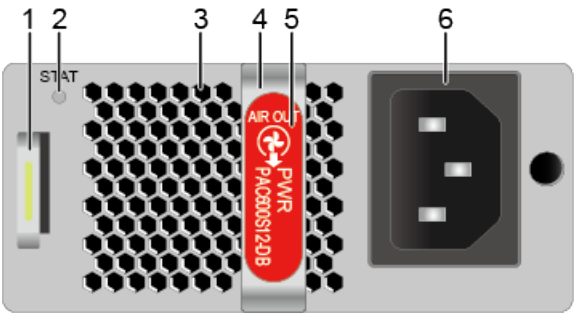
Figure 5-45 Panel of the PAC600S12-DB
