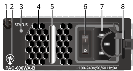
Figure 5-41 Panel of the PAC-600WA-B
