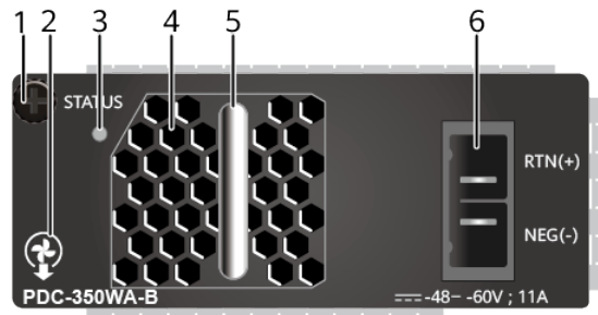
Figure 5-39 Panel of the PDC-350WA-B
