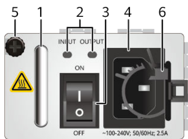
Figure 5-33 Panel of the W0PSA1701
