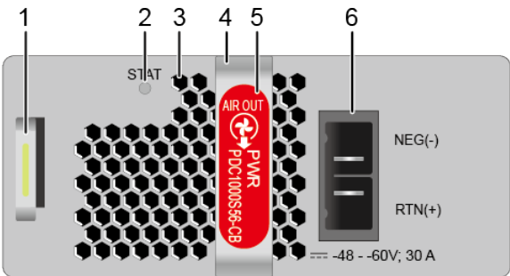
Figure 5-61 Panel of the PDC1000S56-CB
