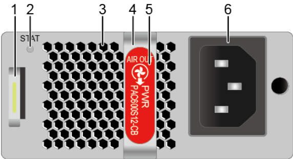
Figure 5-43 Panel of the PAC600S12-CB
