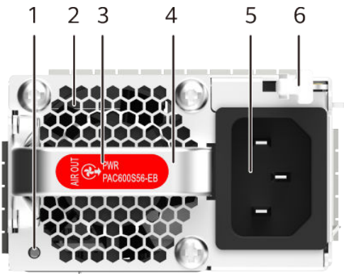
Figure 5-51 Panel of the PAC600S56-EB
