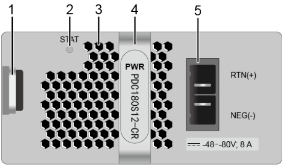
Figure 5-37 Panel of the PDC180S12-CR
